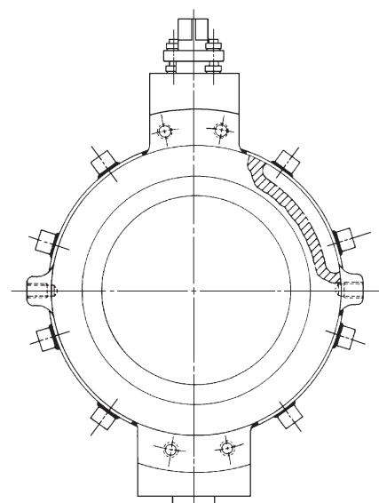
20" (DN 500) Type 815W Valve
