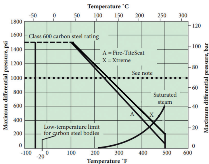
Seat ratings for series 860 valves
