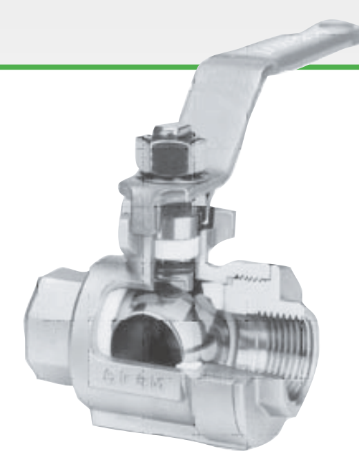
6FR Value-Line™ 1", 2" & 3" series full-bore screwed end ball valves
