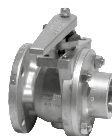
9RFT Full-port flanged ball valves
