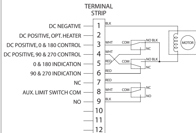
Figure 3 LCU-Series DC Wiring
