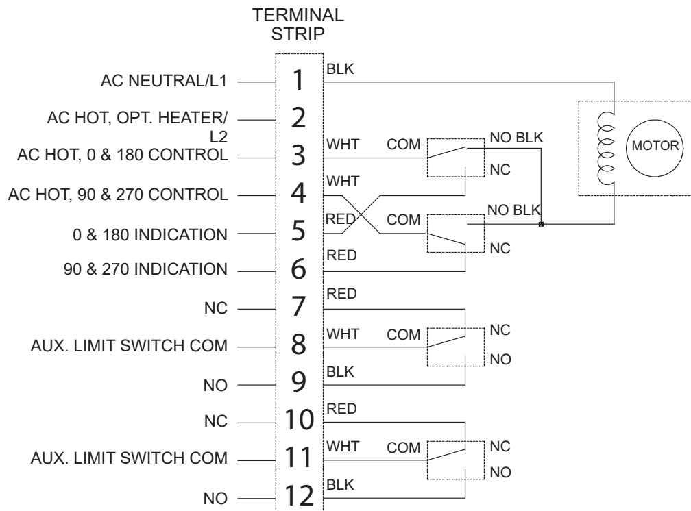
Figure 3A LCU-Series AC Wiring
