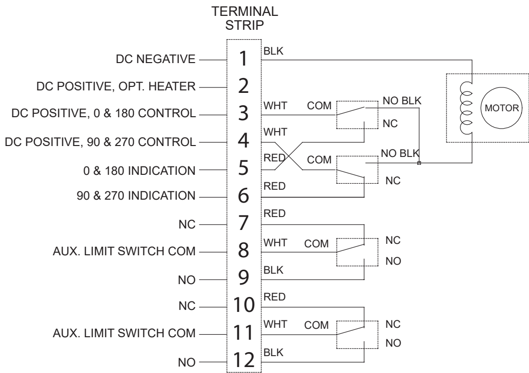
Figure 3B LCU-Series DC Wiring
