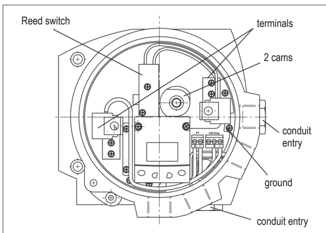
Fig. 46. ND92/93_/R01 layout
