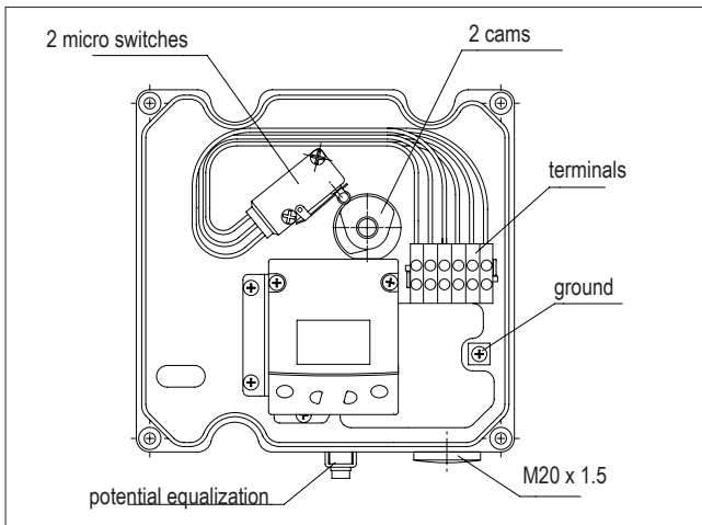
Fig. 40. ND9100_/K0_ layout
