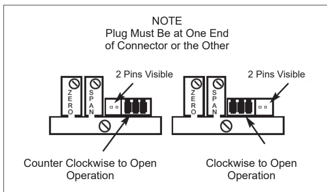
Fig. 50. Plug setting for transmitter operation.
