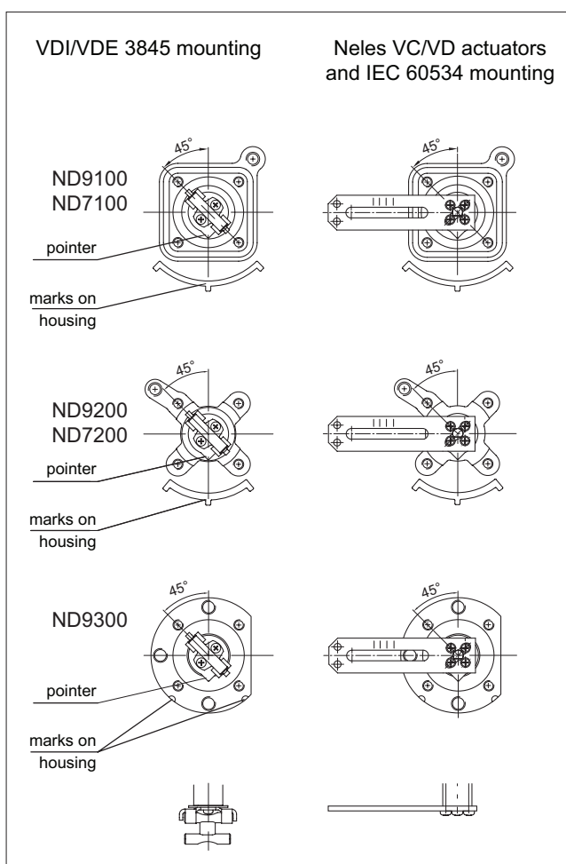
Fig. 4. Shaft coupling alternatives
