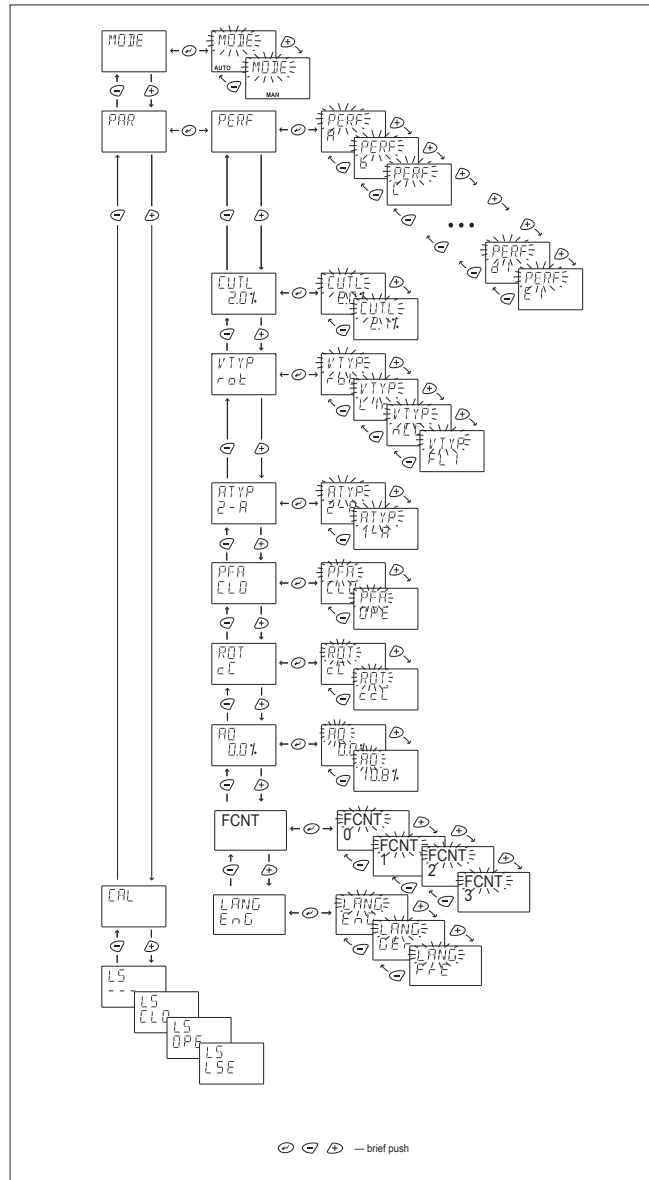
Fig. 21. Configuration, ND9000F
