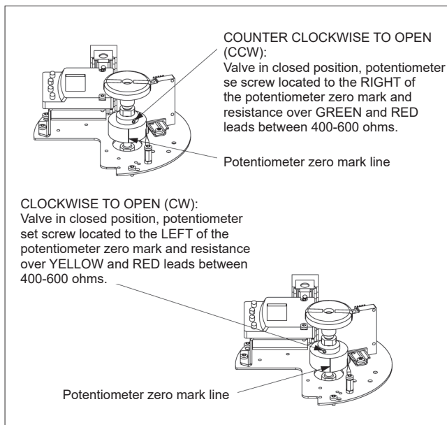
Fig. 49. Potentiometer operation.
