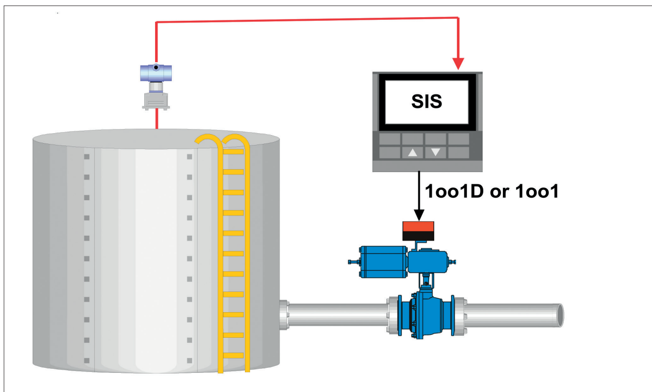
Fig.1. Schematic picture of safety loop. Final element is connected to safety (SIS) logic solver via solenoid or safety valve controller (partial stroke device). This shows single channel final element subsystem with voting 1oo1D or 1oo1.
