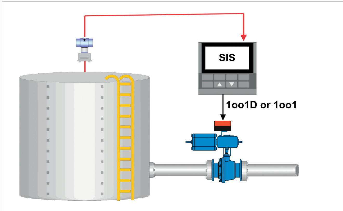
Fig. 1. Schematic picture of safety loop. Final element is connected to safety (SIS) logic solver via solenoid or safety valve controller (partial stroke device). This shows single channel final element subsystem with voting 1oo1D or 1oo1.
