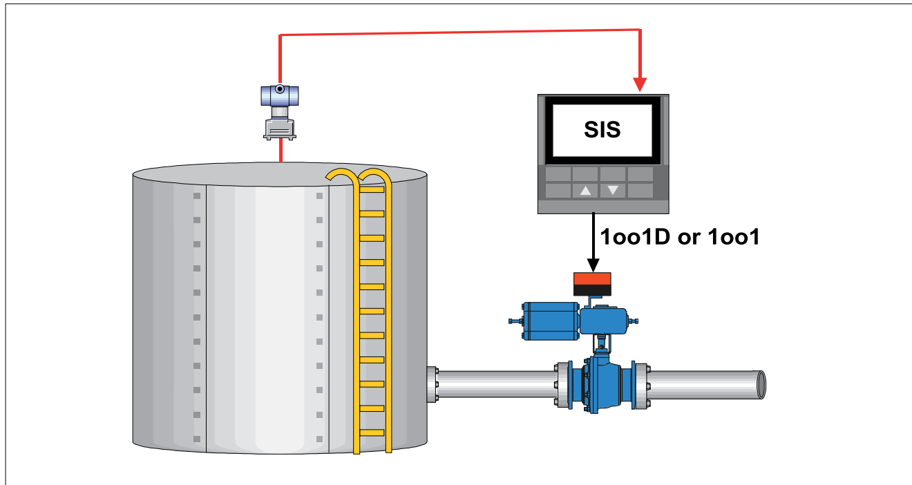
Fig. 1. Schematic picture of safety loop. Final element is connected to safety (SIS) logic solver via solenoid or safety valve controller (partial stroke device). Here shown single channel final element subsystem with voting 1oo1D or 1oo1.
