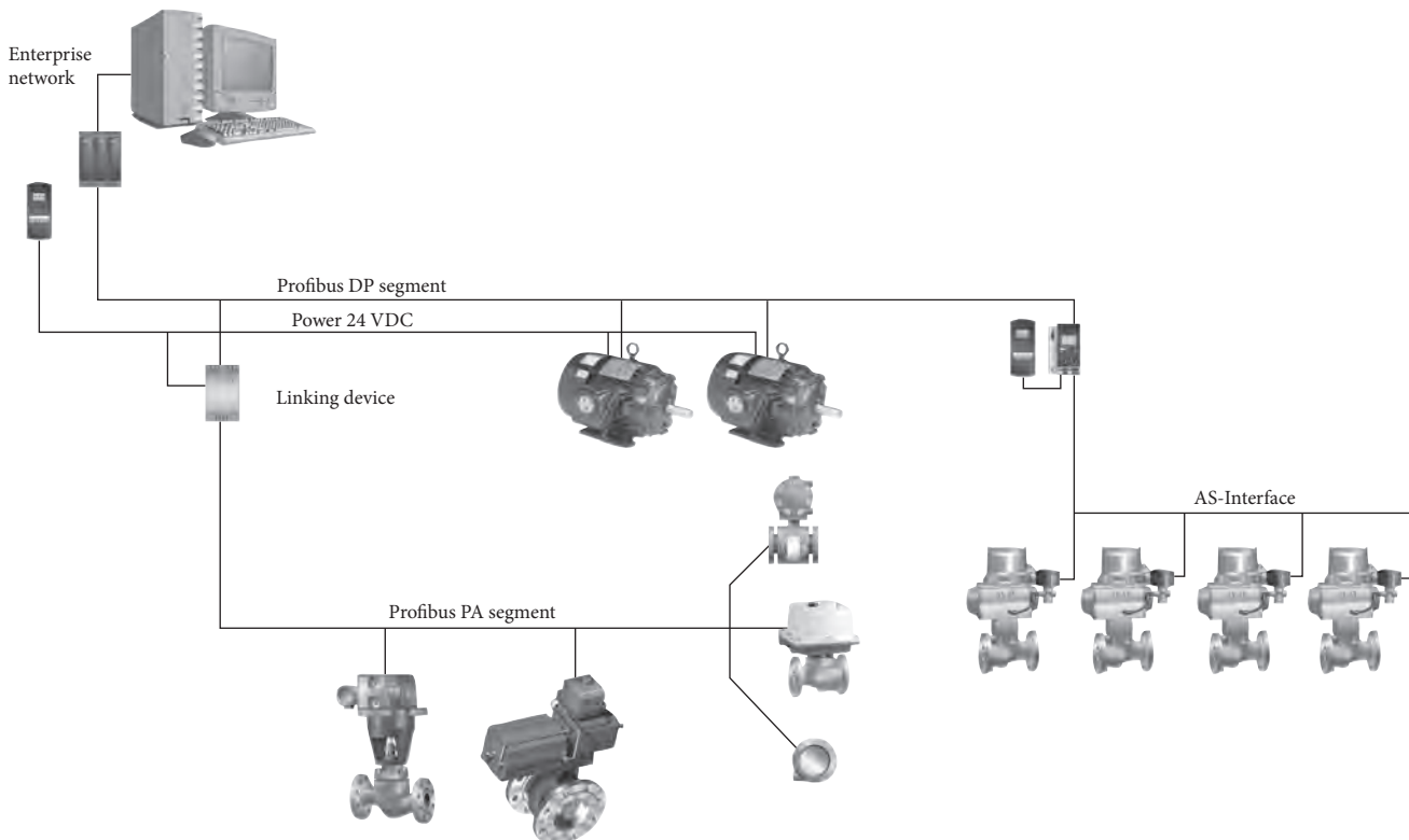
Figure 1 Profibus PA
