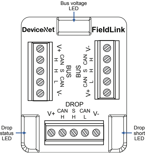
Wiring diagram
