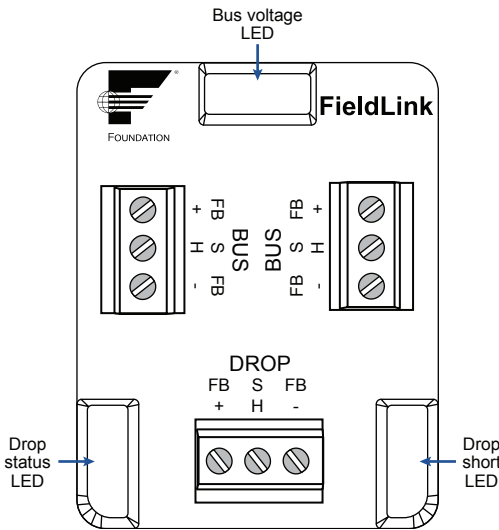
Wiring diagram
