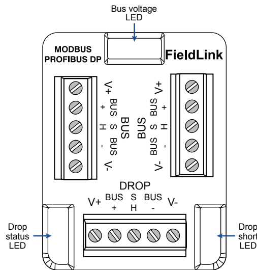
Wiring diagram
