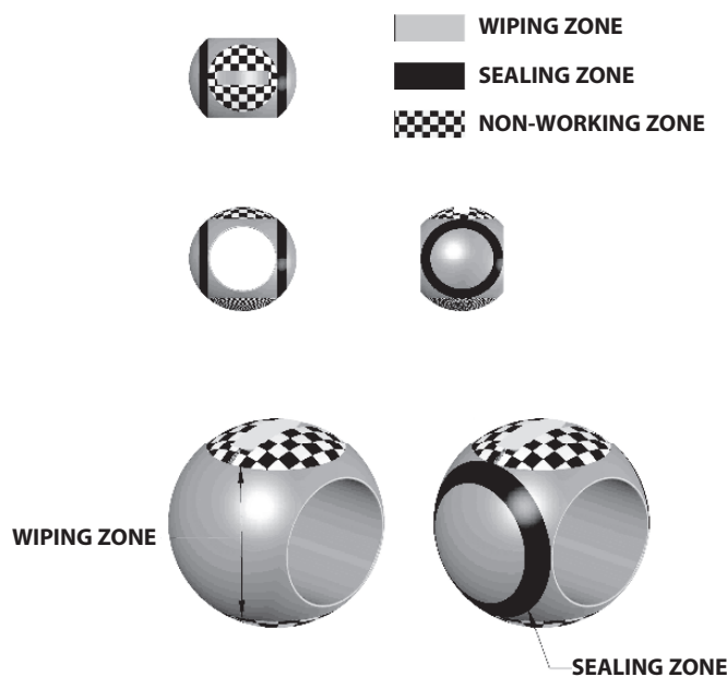
Figure 1: Typical Ball Sealing Area
