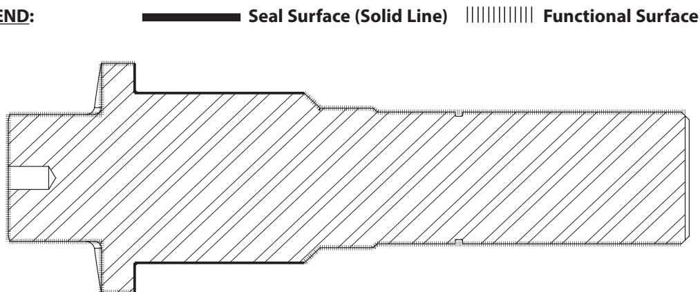
Figure 2: Typical Stem Sealing and Functional Areas
