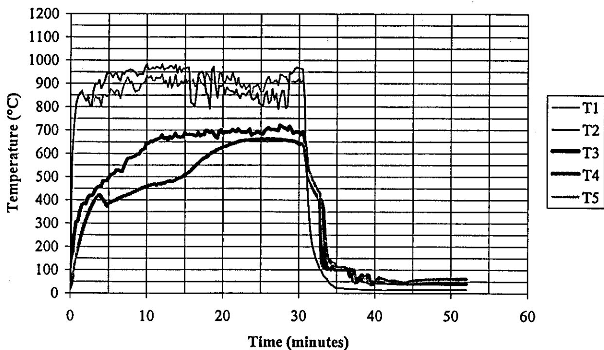
Time-Temperature-graph Valve type: XT08CWTAJ2SJHABA
