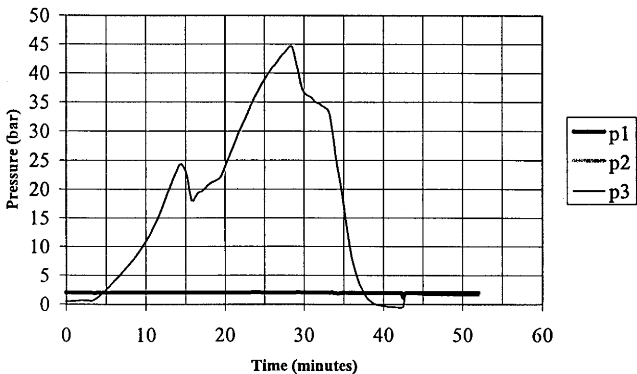
Time-pressure-graph
