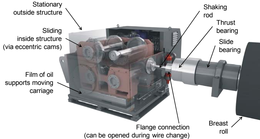
Figure 3. Valmet Breast Roll Shaker's compact design uses balanced eccentric mass pairs to shake the breast roll in the cross-direction.
